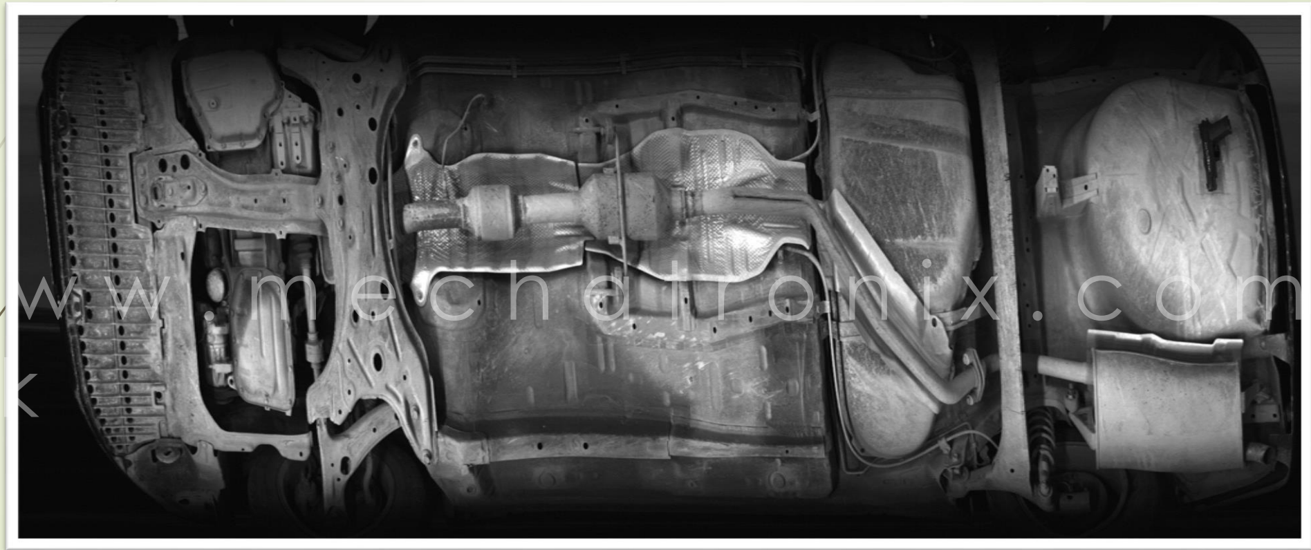
UVSS Scanned Image
