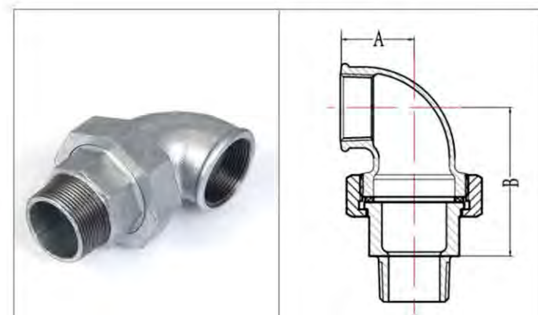
Fig.98 M&F Conical Union Elbow
