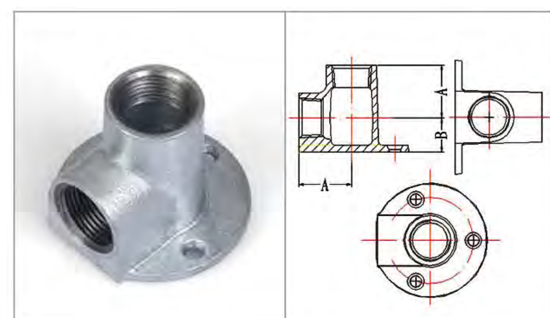
Fig.1221 Banded Side Outlet Elbow
