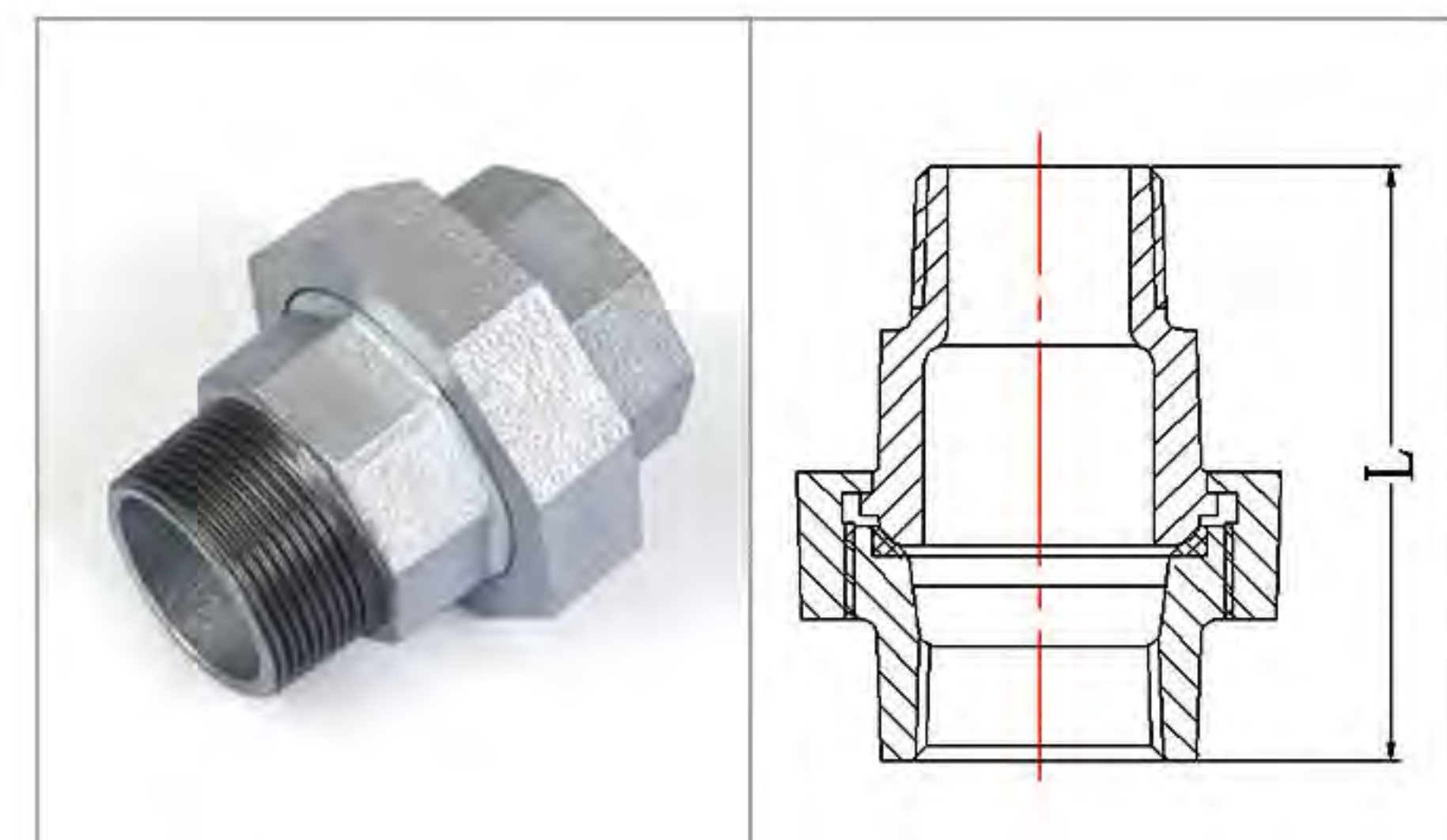
Fig.343 Brass Unions, Taper Seat, M&F
