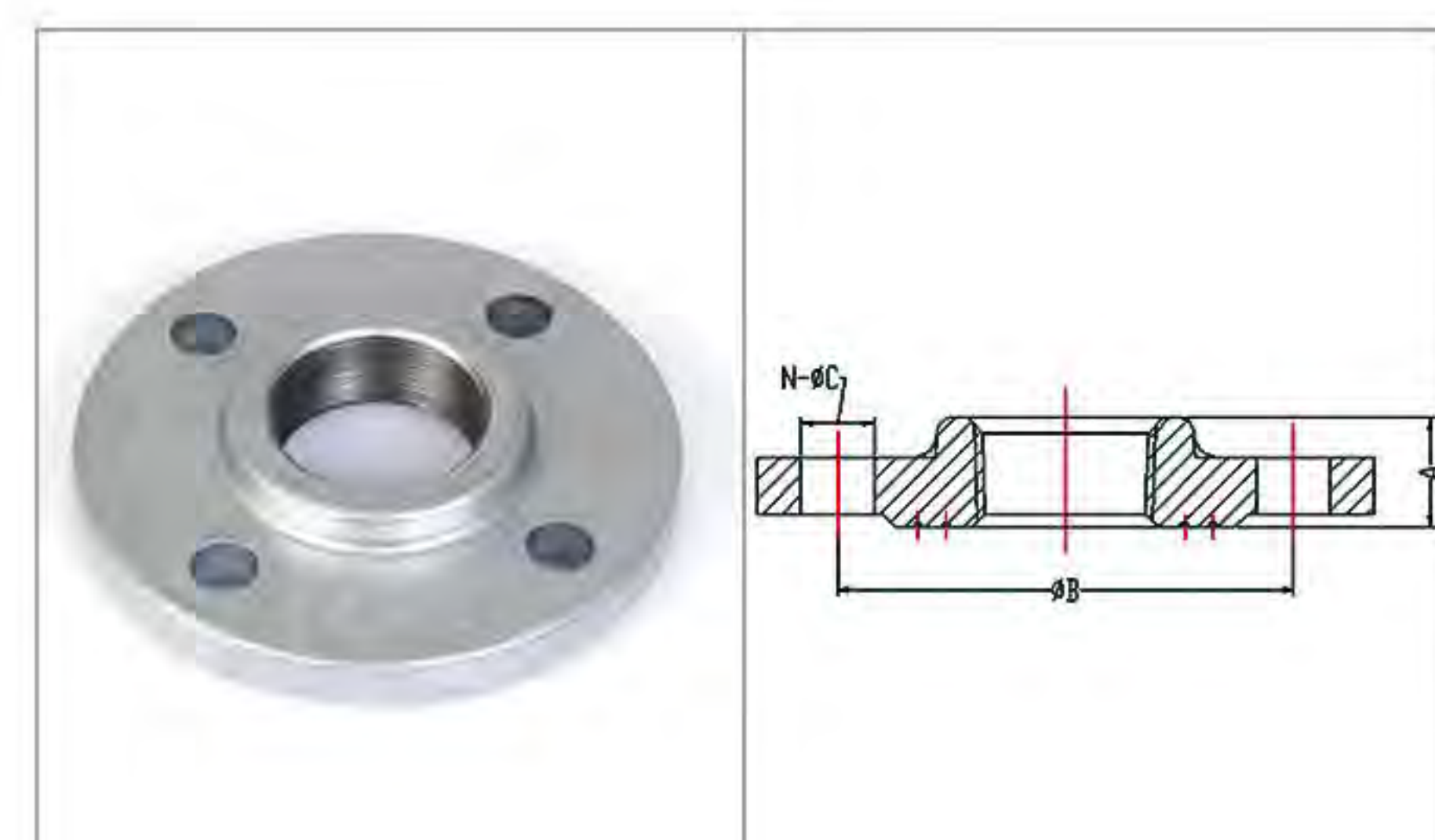
Fig.329 Round Flange With 4 Bolt HoleS
