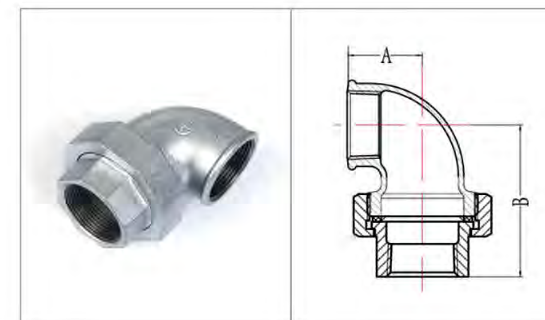
Fig.96 Union Elbow, conical seat
