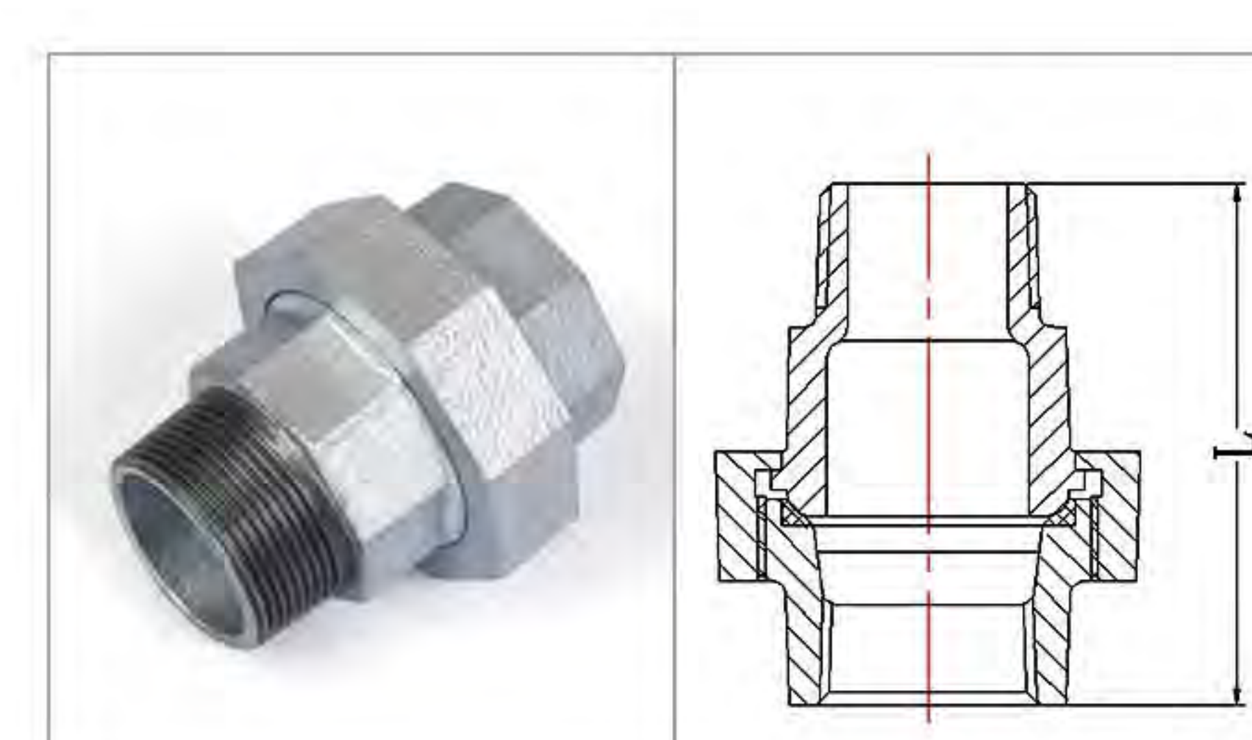
Fig.341 Union,conical seat,M&F
