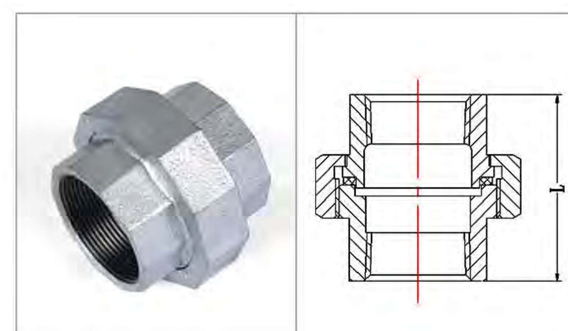
Fig.340 Union,conical seat
